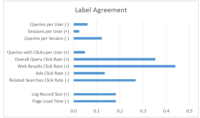
Figure 5. The Label Agreement of Common Search Metrics
