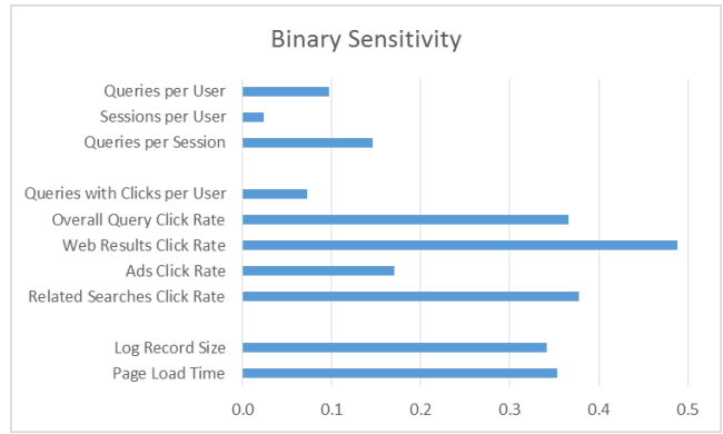
Figure 4. The Sensitivity of Common Search Metrics
