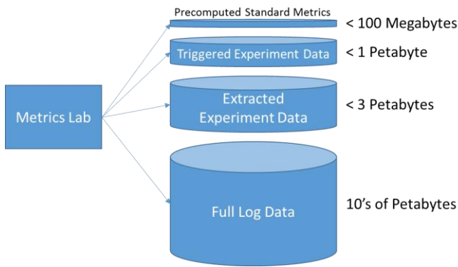
Figure 2. Cache structure for Metrics Lab
